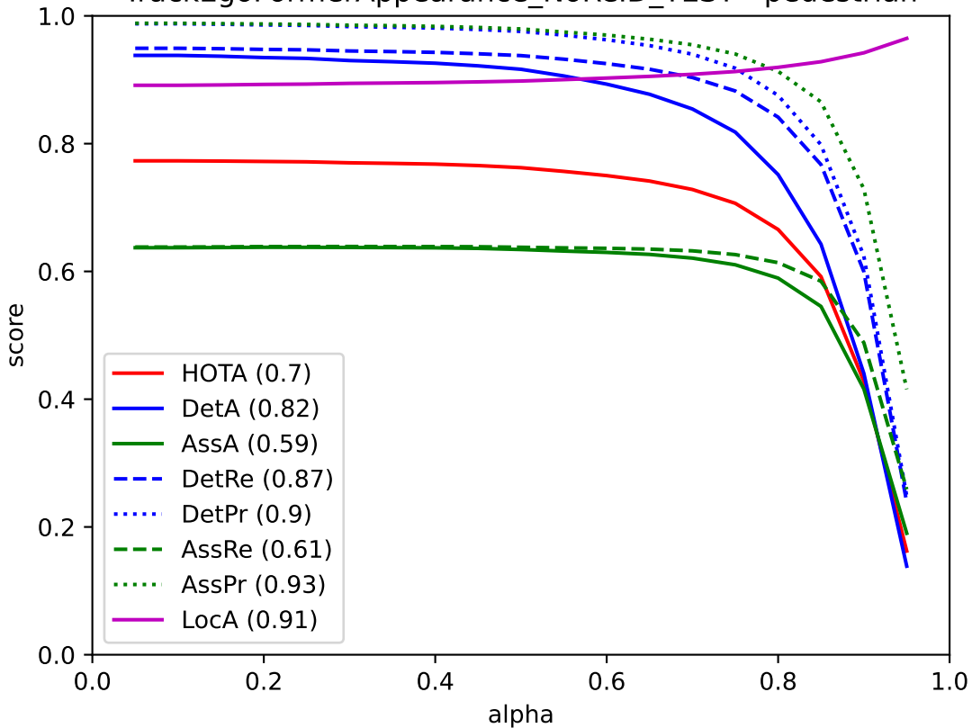
TrackEgoFormerAppearance_NoReID_TEST - pedestrian
