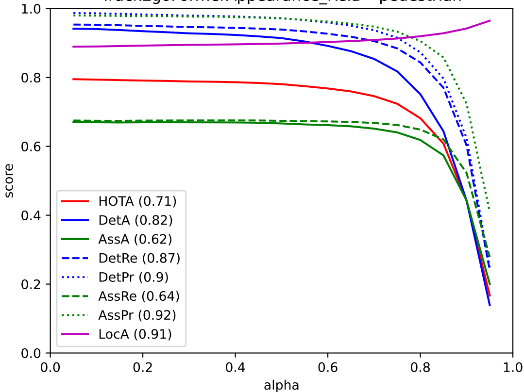
TrackEgoFormerAppearance_ReID - pedestrian
