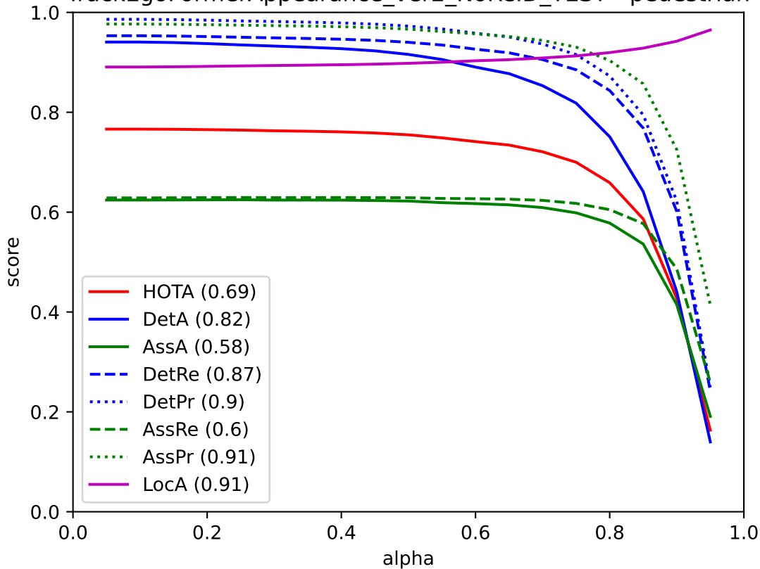
TrackEgoFormerAppearance_ver2_NoReID_TEST - pedestrian
