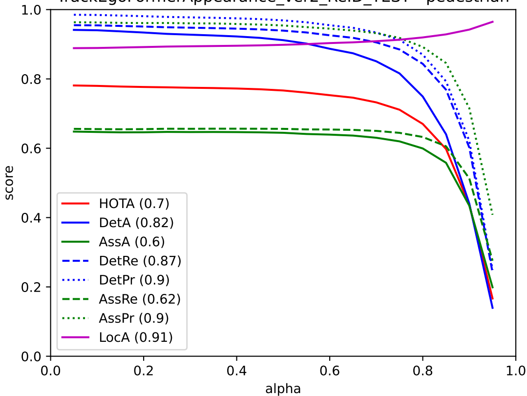
TrackEgoFormerAppearance_ver2_ReID_TEST - pedestrian
