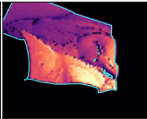
(b) Support S
