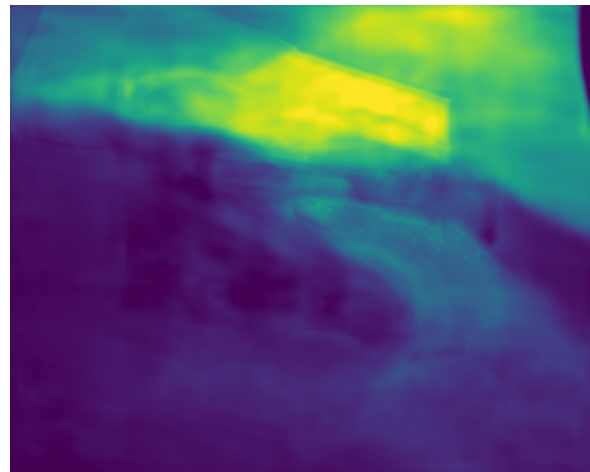
\mathbf{D}_t^{\text{syn}}
