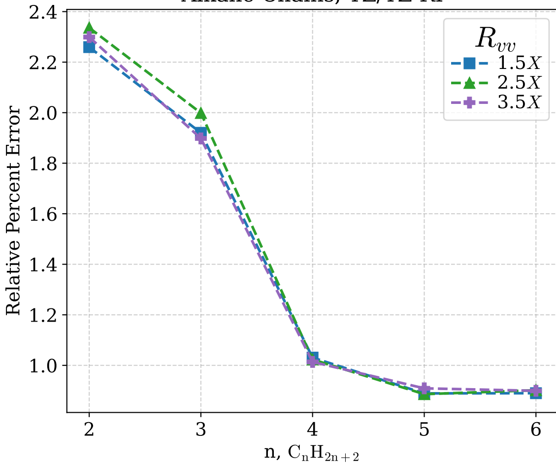
Lov_aa L_2 Error vs System Size Alkane Chains, TZ/TZ-RI
