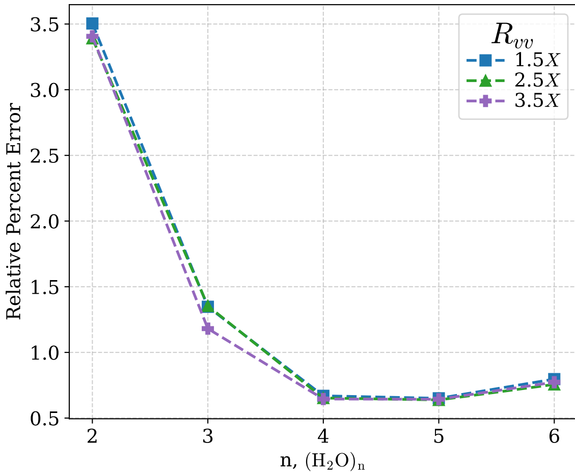
Lov_aa L_2 Error vs System Size Water Clusters, TZ/TZ-RI
