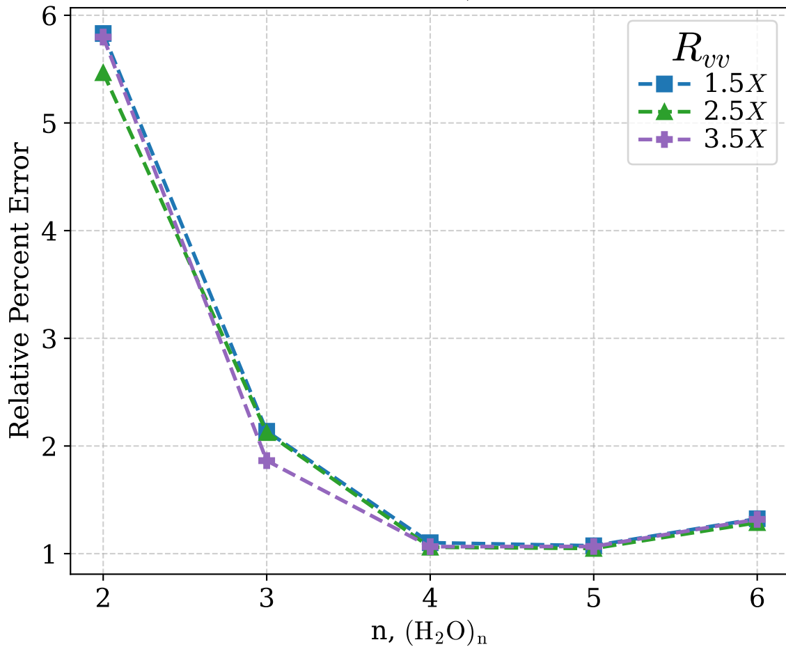
Lov_ai L_2 Error vs System Size Water Clusters, TZ/TZ-RI
