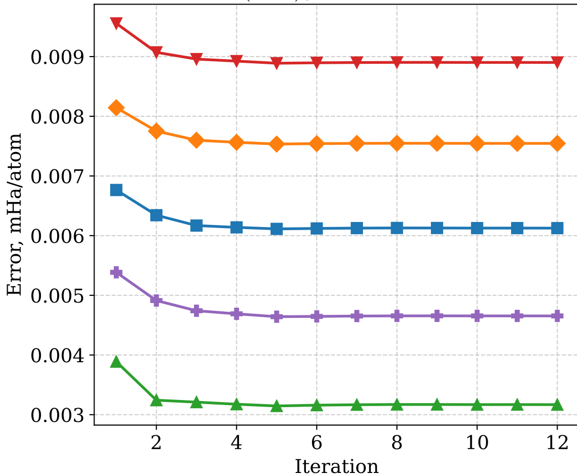
HL Error per Iteration (H 2 O) 6 , DZ/DZ-RI
