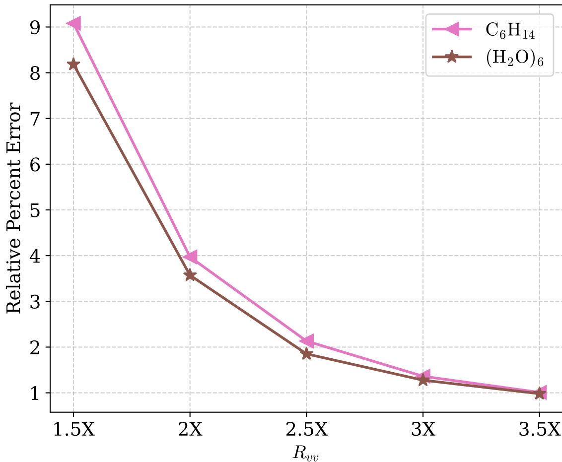
Lvv_ii L_2 Percent Error vs Rank TZ/TZ-RI
