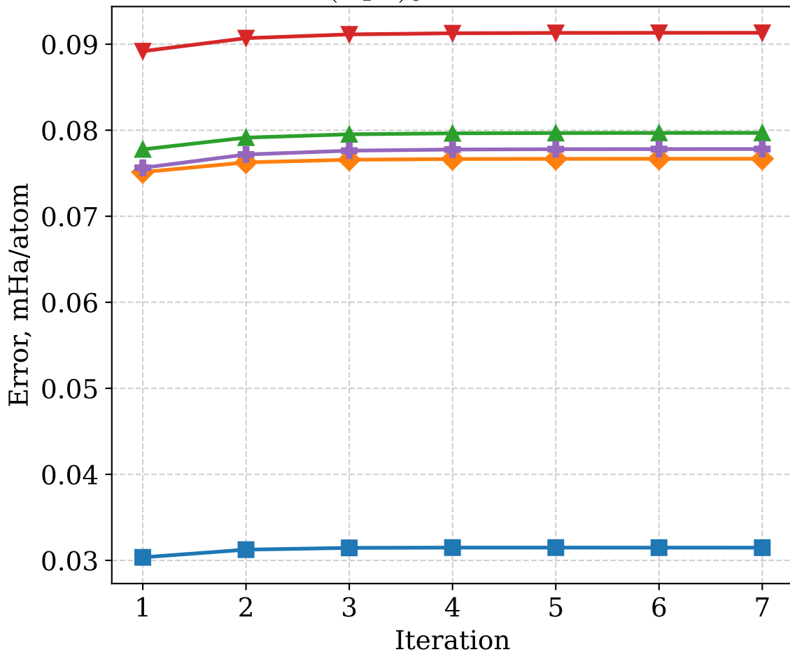
MPCC Error per Iteration (H 2 O) 6 , TZ/TZ-RI
