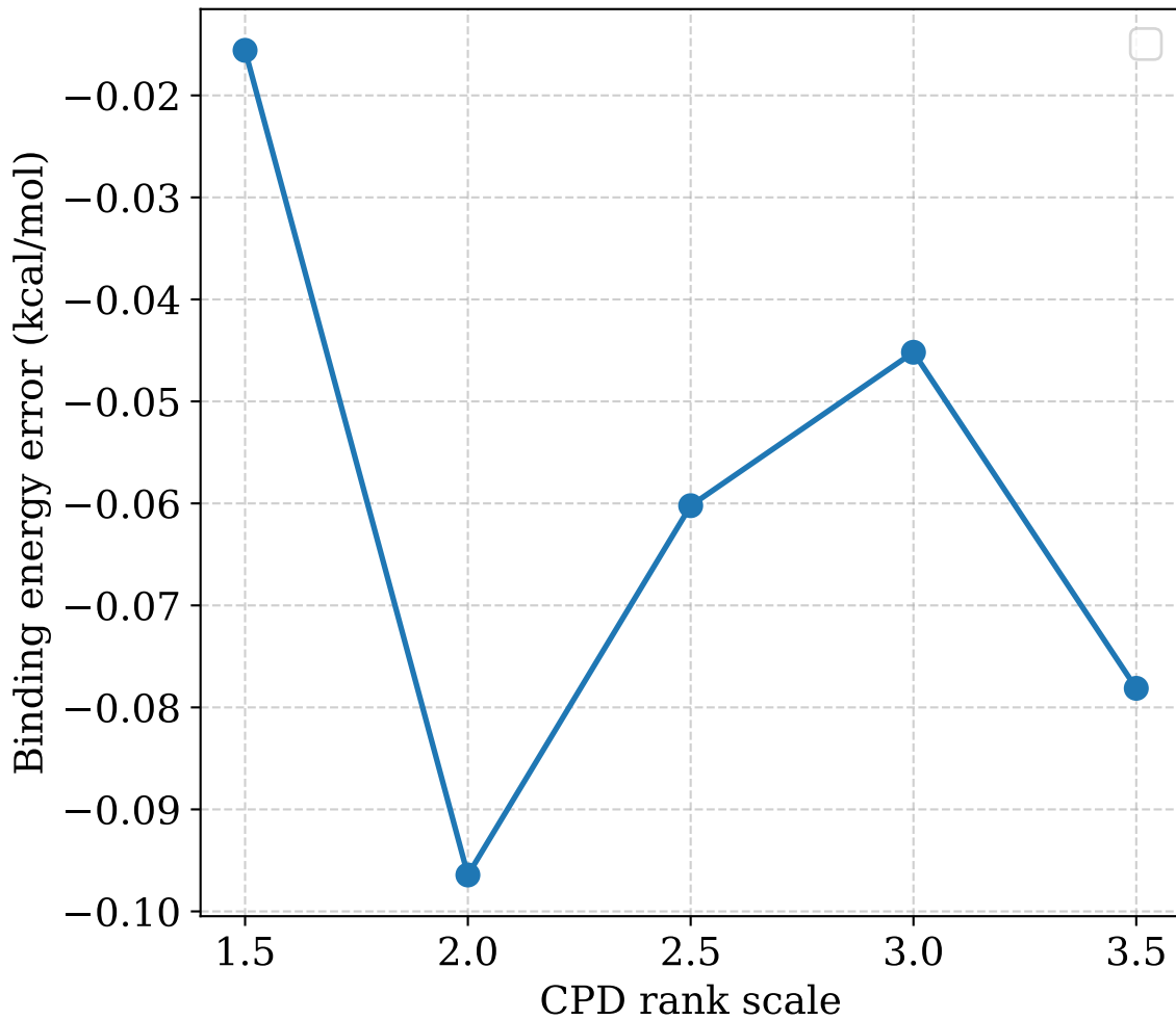
CH 4 (H 2 O) 4 binding energy error (cc-pvtz)
