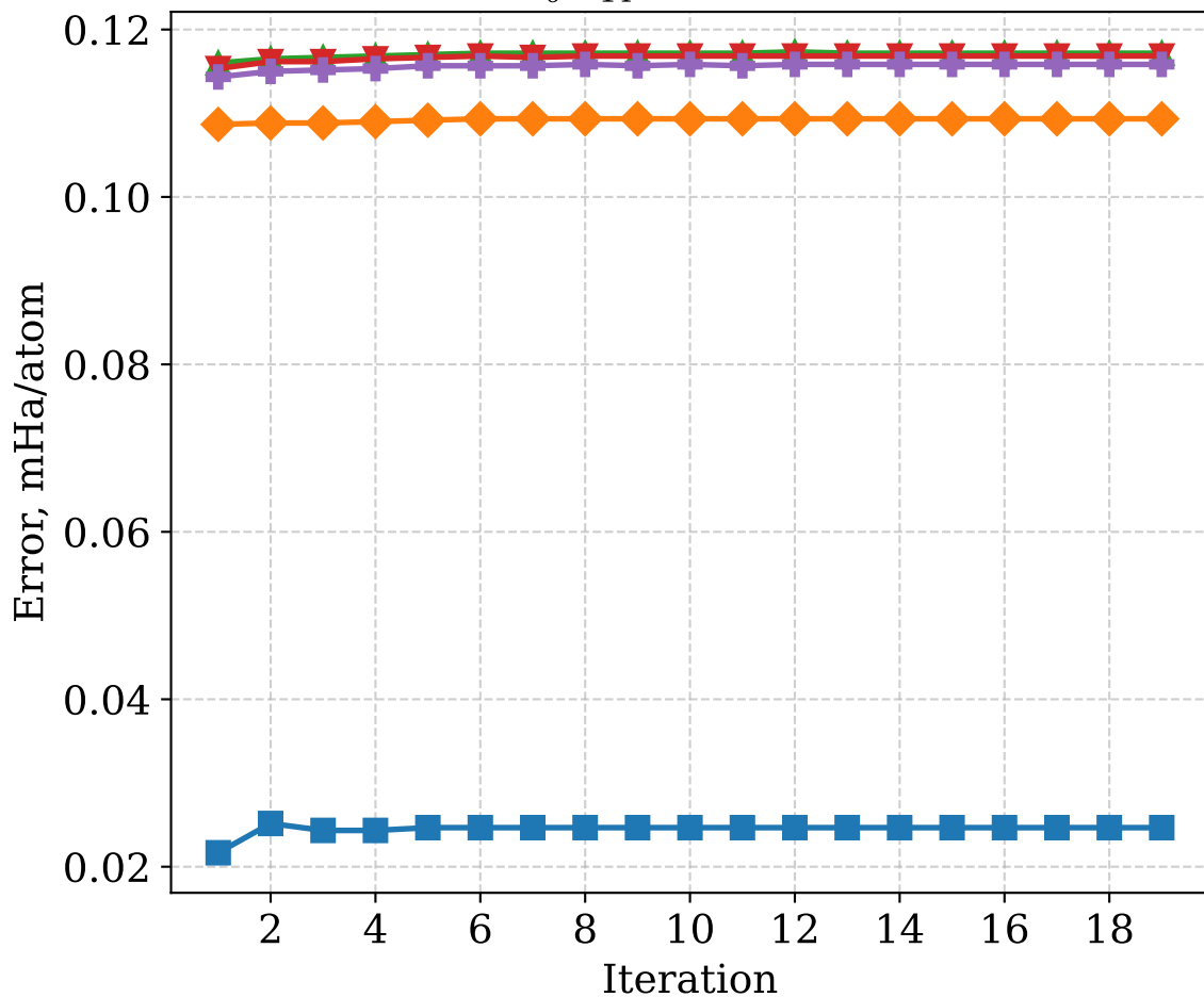
LL Error per Iteration \text{C}_6\text{H}_{14} , TZ/TZ-RI
