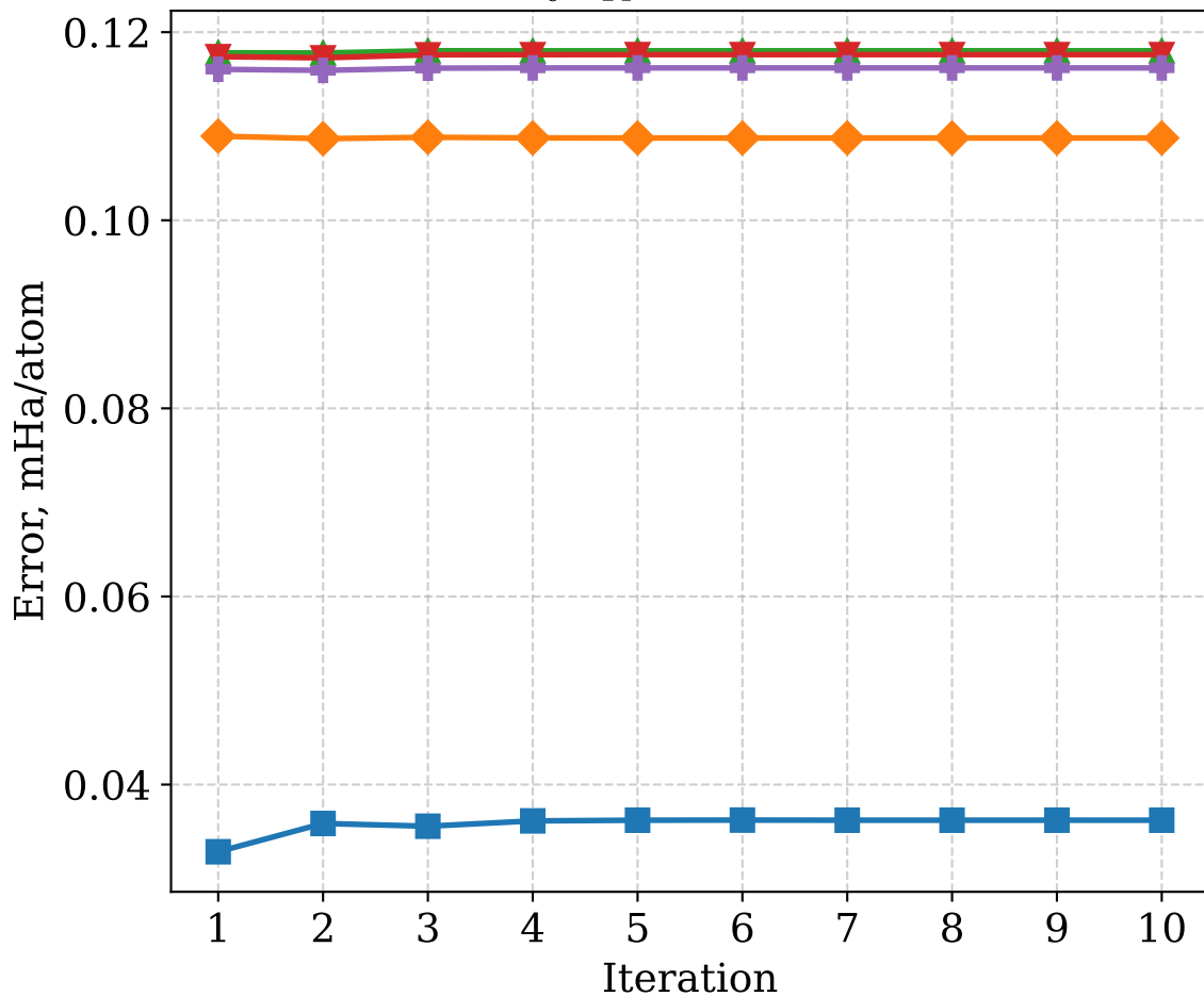
HL Error per Iteration \text{C}_6\text{H}_{14} , TZ/TZ-RI
