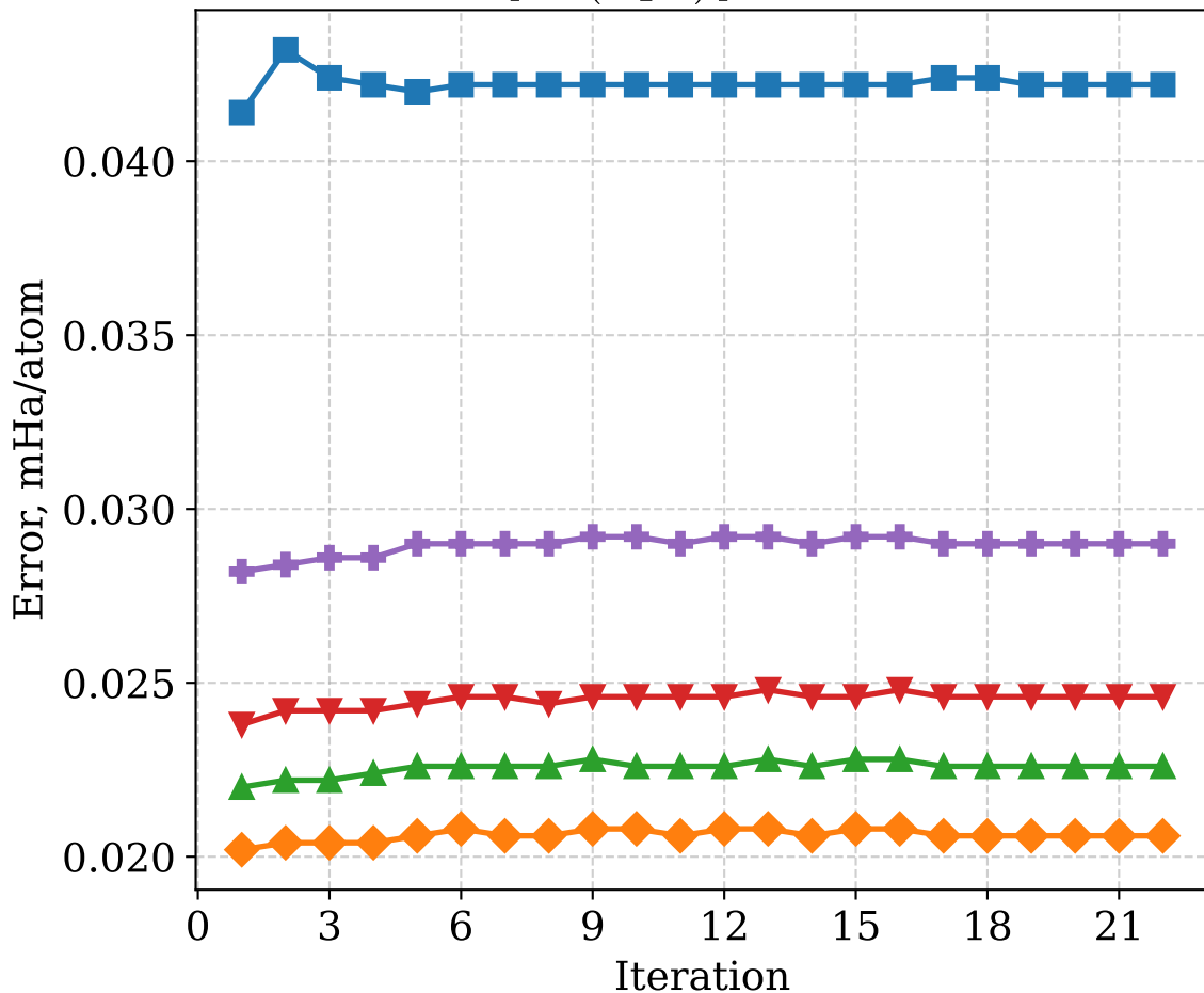
LL Error per Iteration \text{CH}_4 \dots (\text{H}_2\text{O})_4 , TZ/TZ-RI
