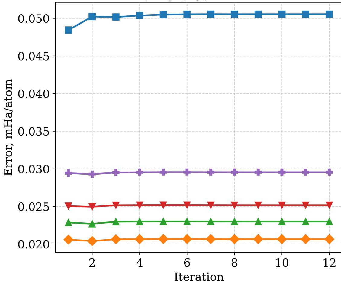
HL Error per Iteration \text{CH}_4 \dots (\text{H}_2\text{O})_4 , TZ/TZ-RI
