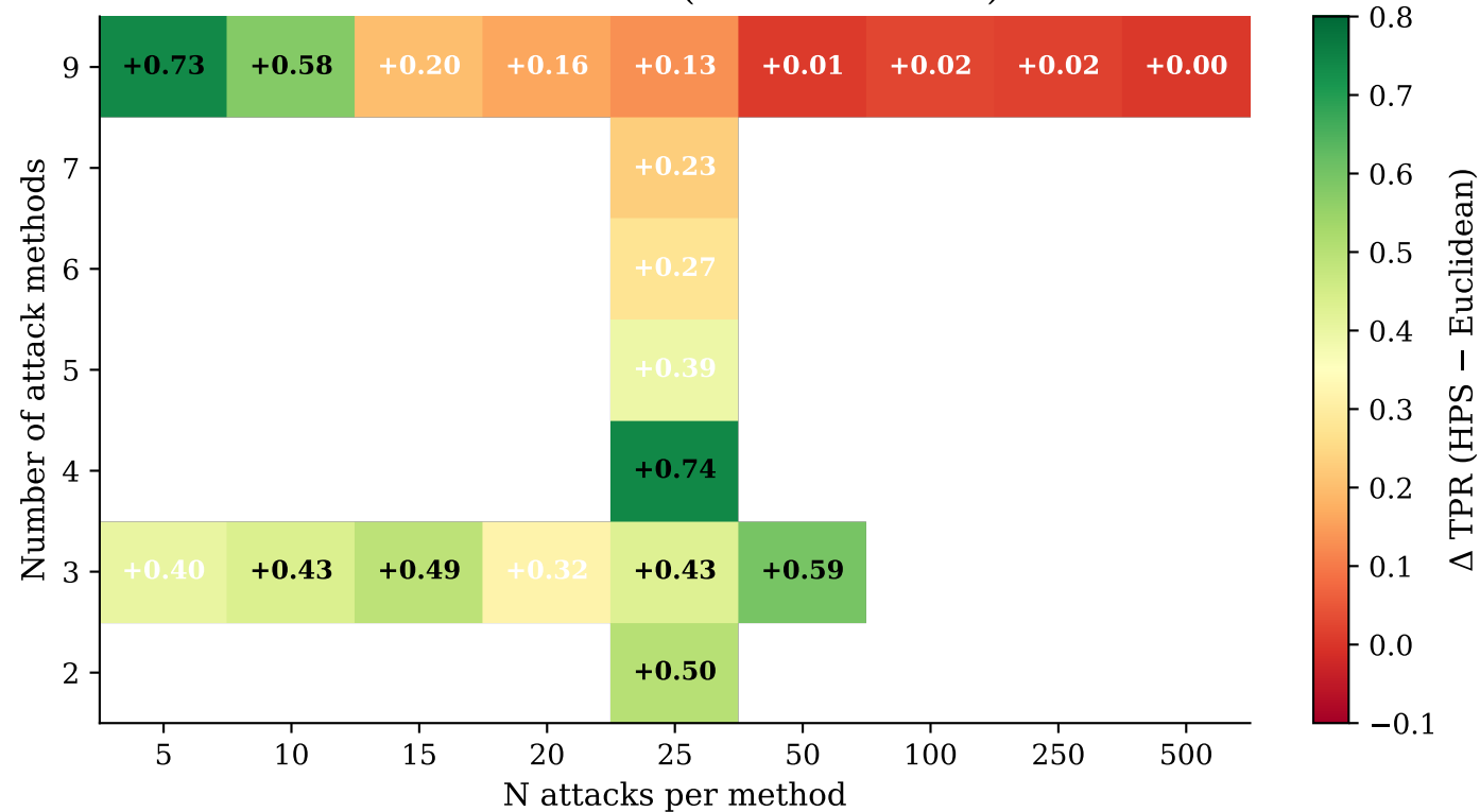
HPS - Euclidean \Delta (cross-attack TPR)
