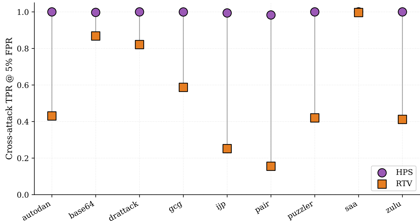
HPS vs RTV — Per-Attack Cross-Attack Performance
