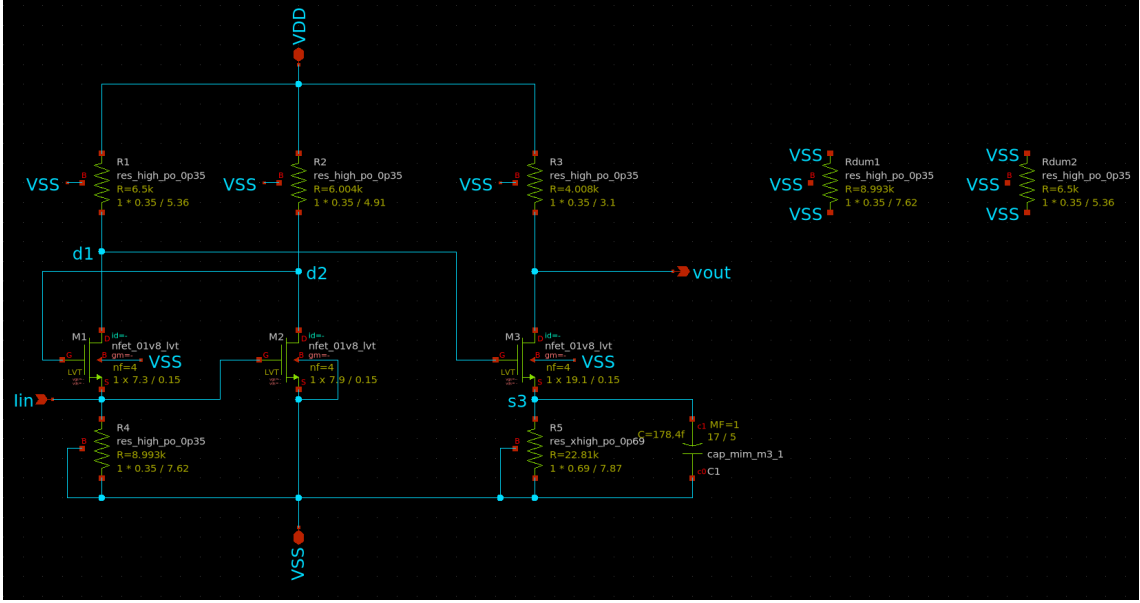
Figure 10: RGC-CD TIA captured in xschem : signal devices M_1 – M_3 ( nfet_01v8_lvt , n_f = 4/4/4 ), the R_1 – R_5 poly-resistor bias network with two flanking dummies, and the MIM degeneration capacitor C_1 . This schematic drives both the pre-layout simulation and the LVS comparison.
