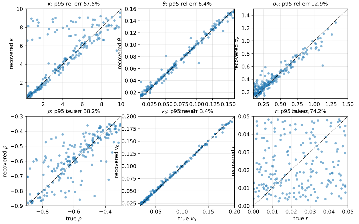
Figure 6: Recovered versus true parameters on the 200-surface MC reference after a flat-init Adam inversion of the surrogate. Dashed lines are the identity. Per-parameter p_{95} relative errors are reported in the titles.
