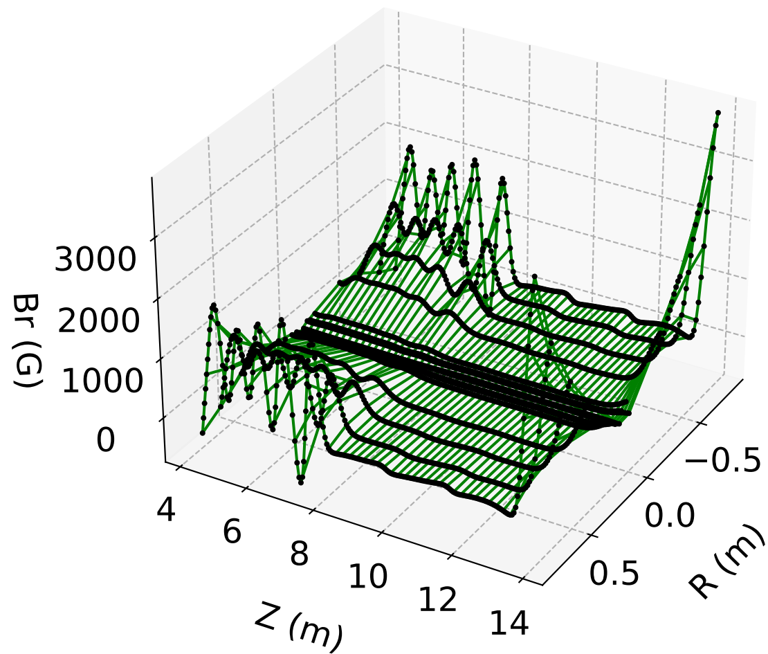
B_r vs. r, z ( \phi = 0 ) LSQ Refit (#1)
