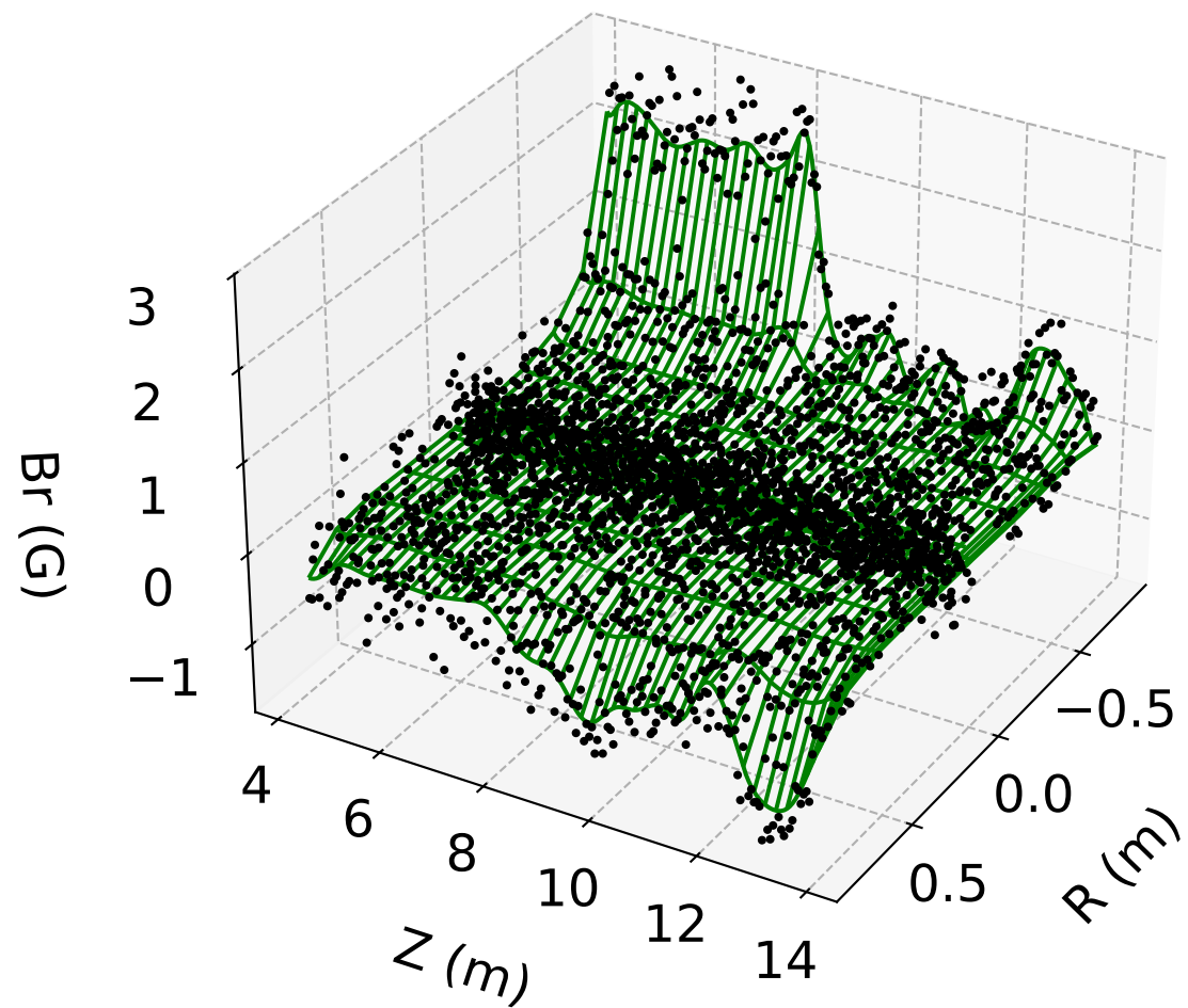
B_r vs. r, z ( \phi = 0 ) PINN Model (#1)
