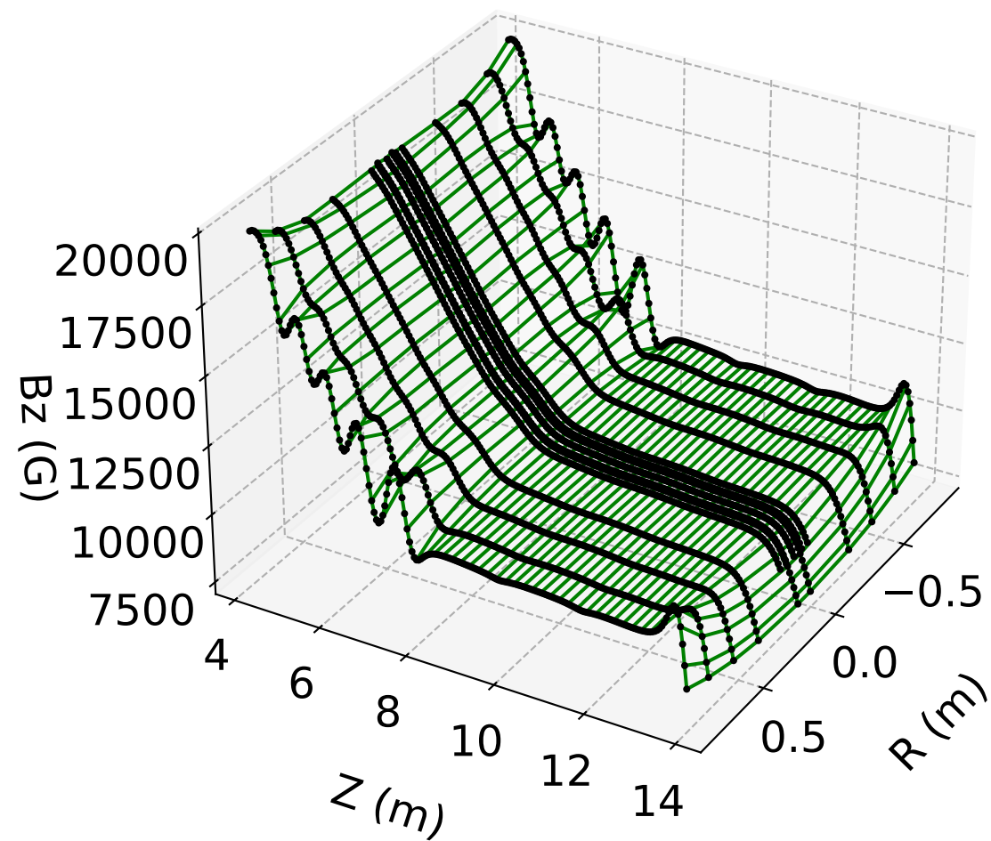
B_z vs. r, z ( \phi = 0 ) LSQ Refit (#1)
