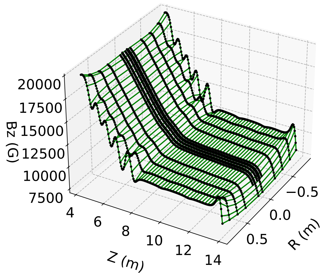
B_z vs. r, z ( \phi = 0 ) LSQ Model (#1)
