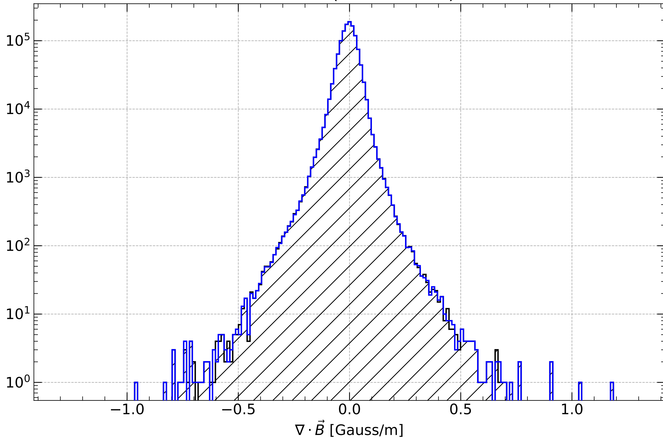
PINN \nabla \cdot \vec{B} (Test Dataset)
