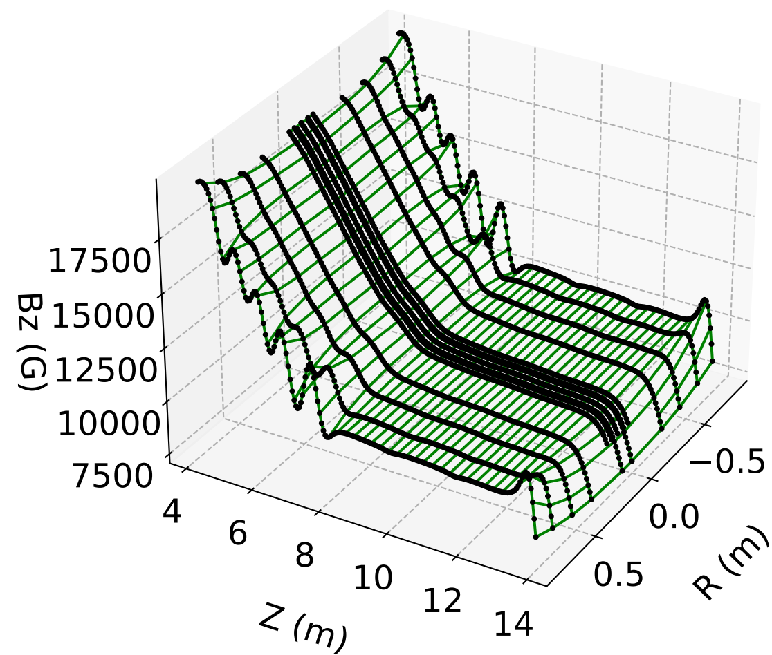
B_z vs. r, z ( \phi = 0 ) LSQ Model (#2)
