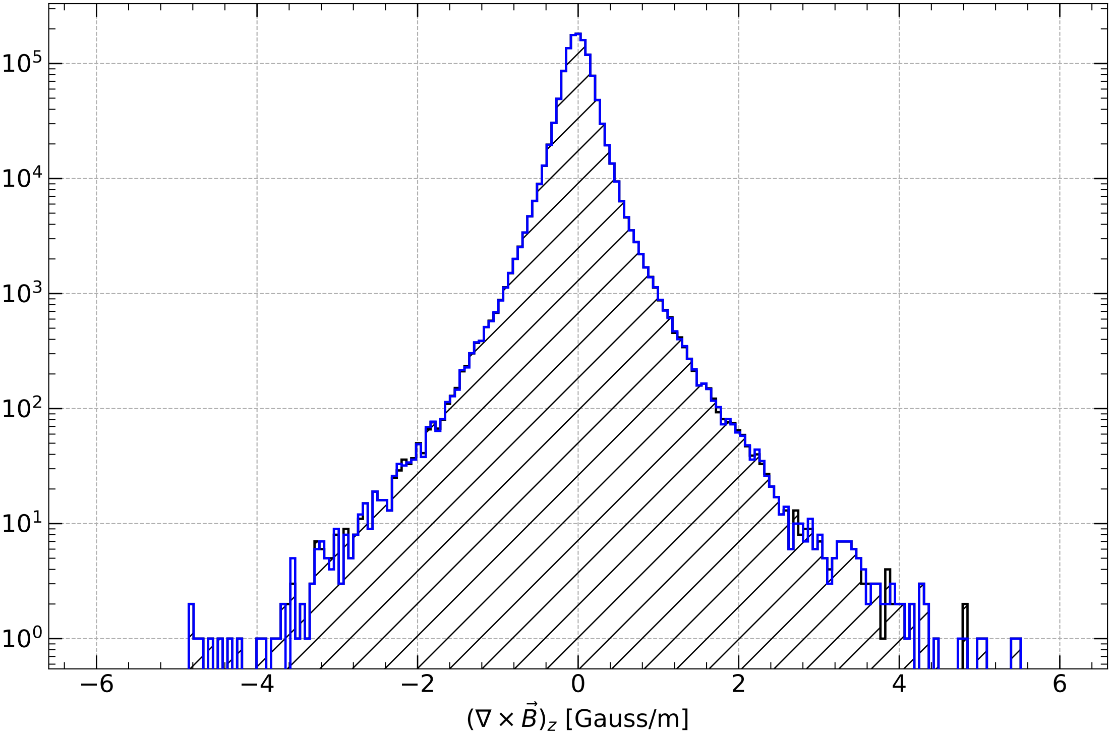
PINN (\nabla \times \vec{B})_z (Test Dataset)
