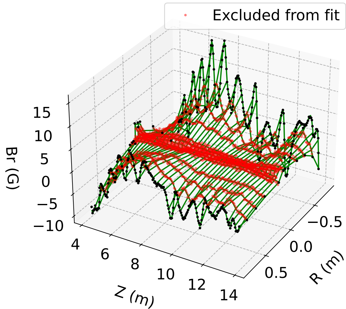
B_r vs. r, z ( \phi = 0 ) PINN Model (#3)
