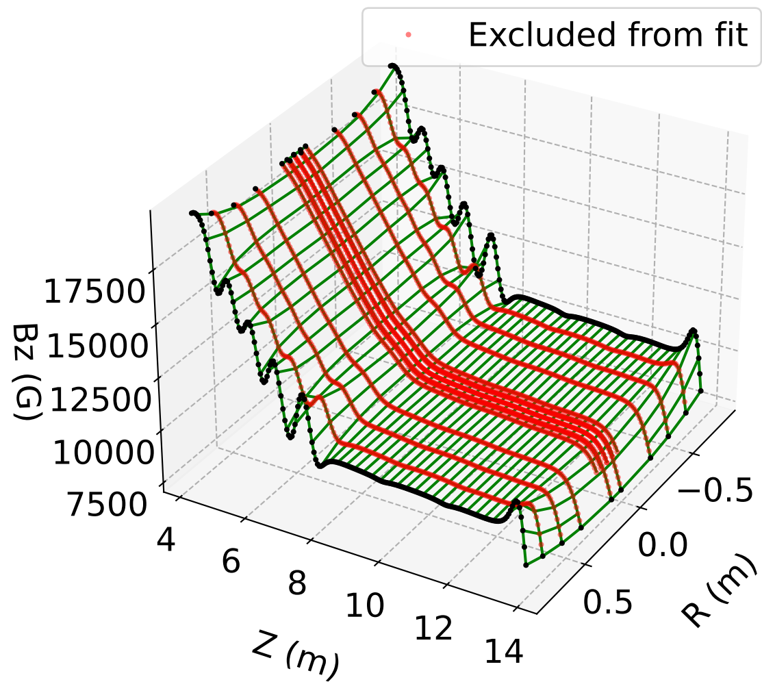
B_z vs. r, z ( \phi = 0 ) Full Model (#3)
