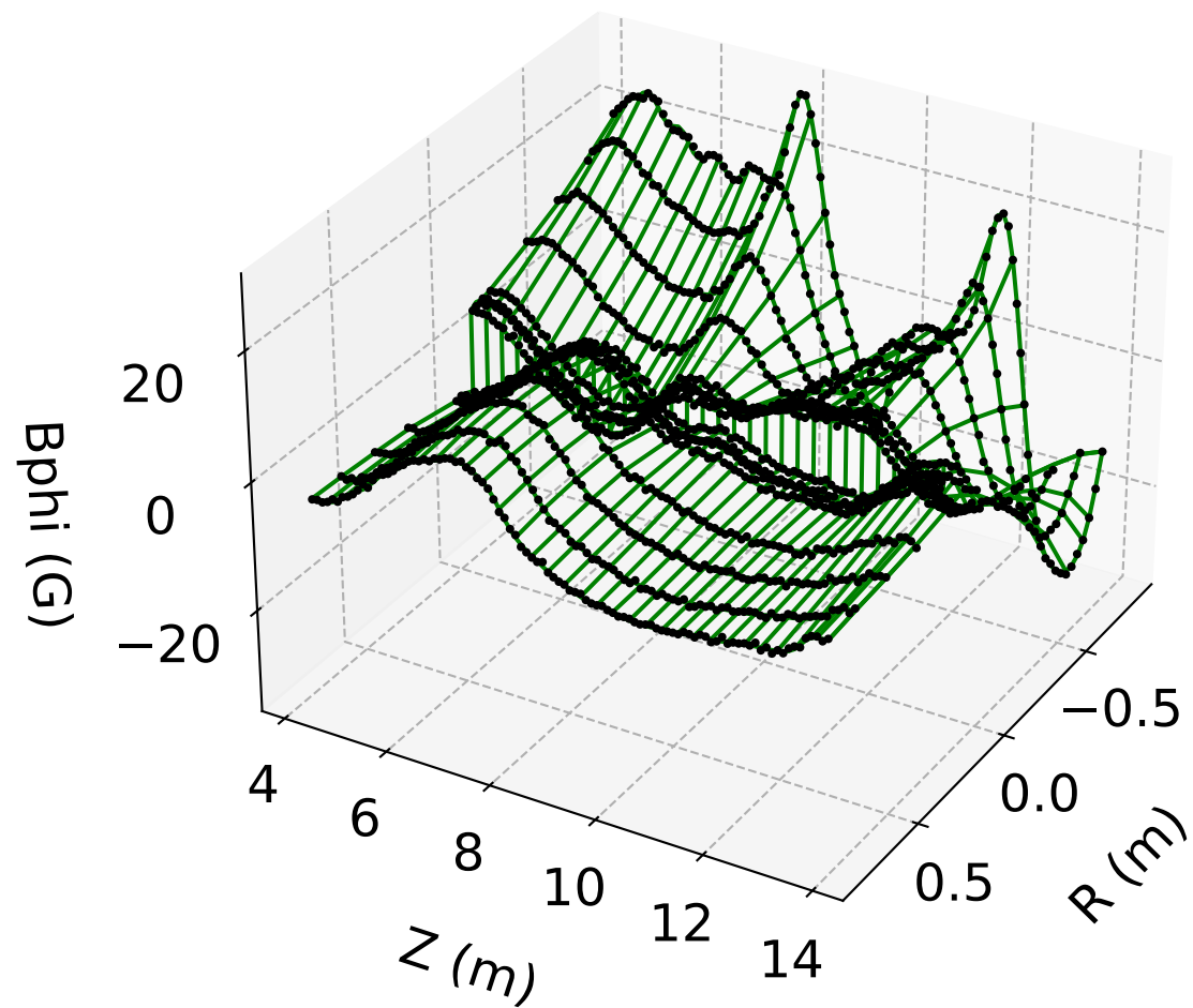
B_\phi vs. r, z ( \phi = 0 ) Full Model (#9)
