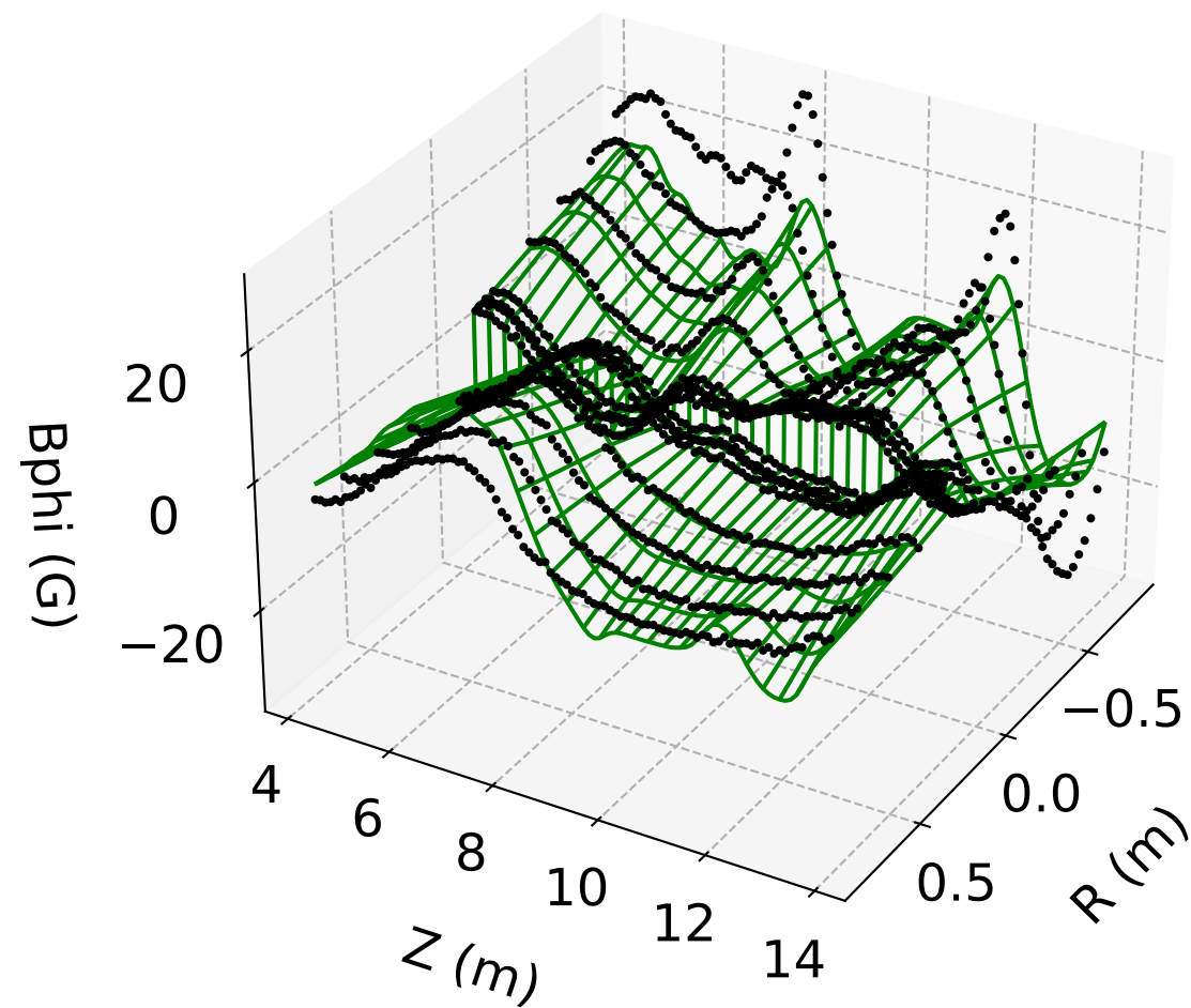
B_\phi vs. r, z ( \phi = 0 ) LSQ Model (#9)
