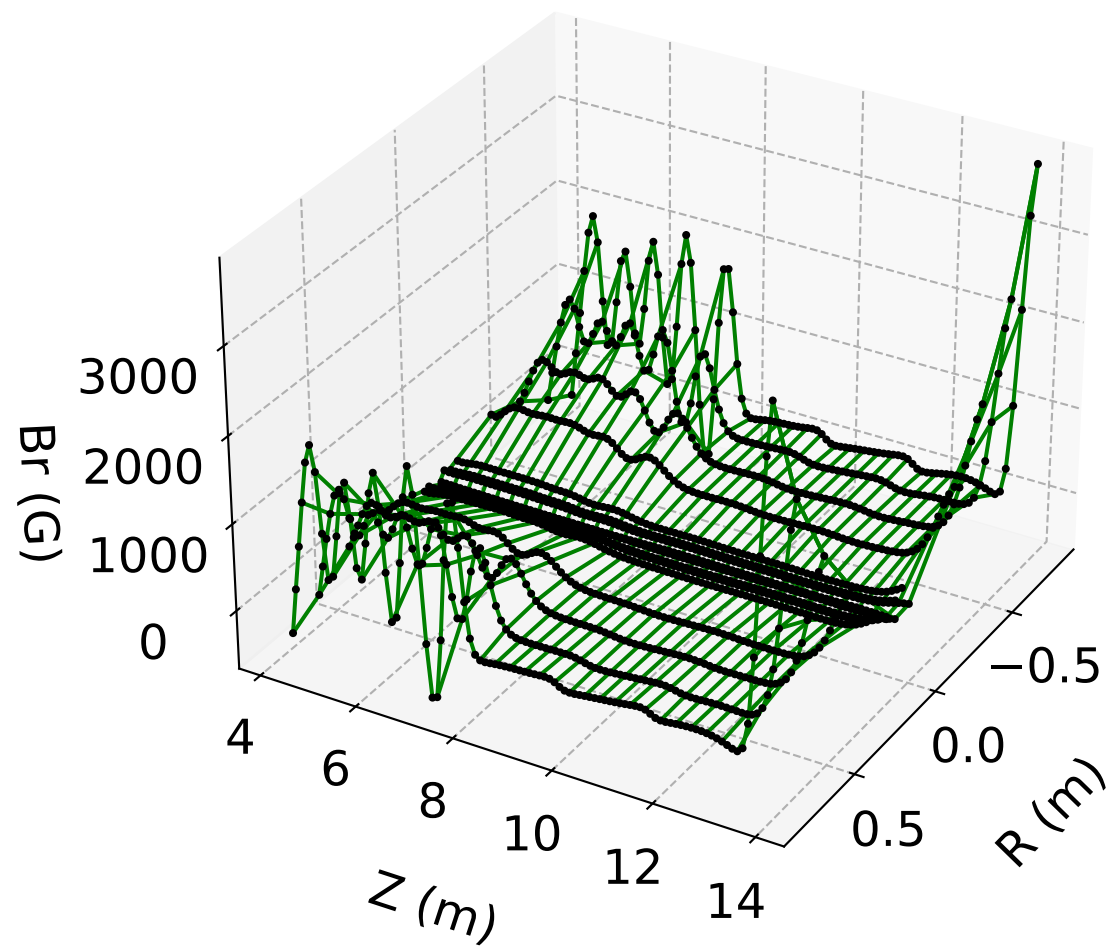
B_r vs. r, z ( \phi = 0 ) Full Model (#9)
