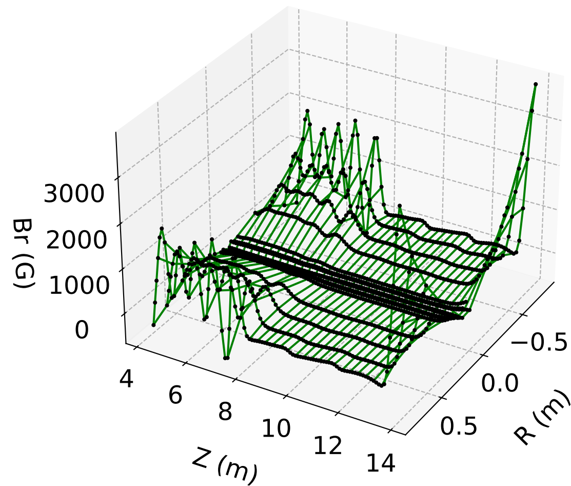
B_r vs. r, z ( \phi = 0 ) LSQ Model (#9)
