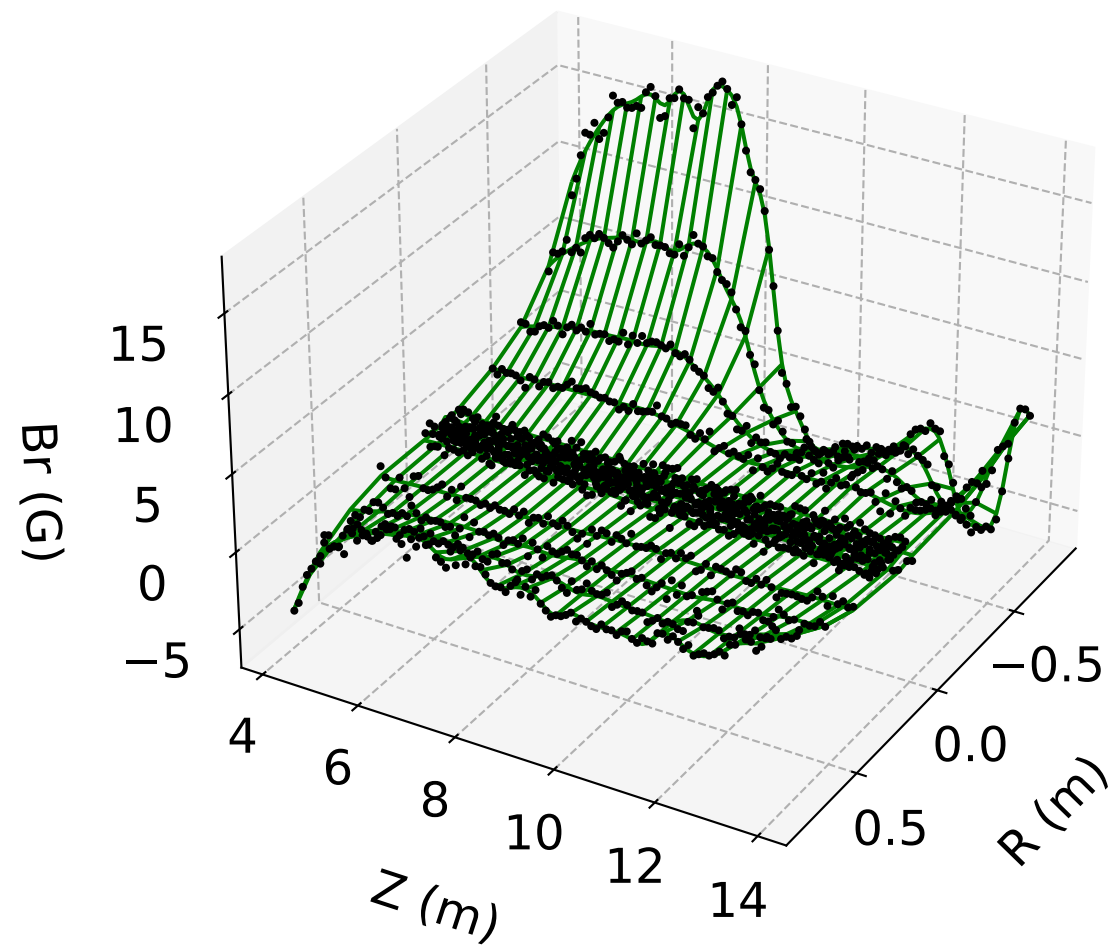
B_r vs. r, z ( \phi = 0 ) PINN Model (#9)
