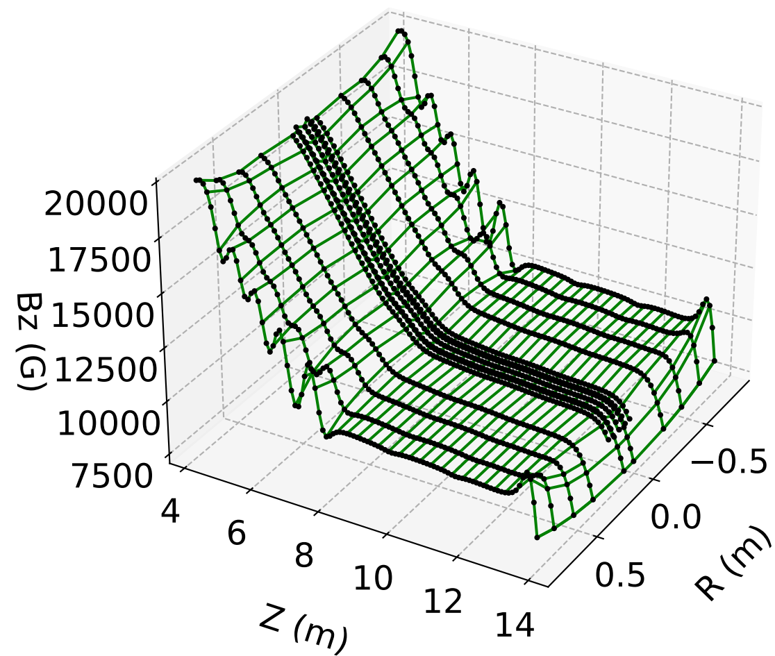
B_z vs. r, z ( \phi = 0 ) Full Model (#9)
