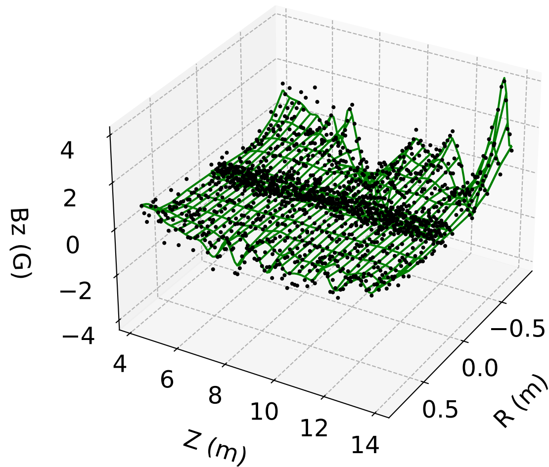
B_z vs. r, z ( \phi = 0 ) PINN Model (#9)
