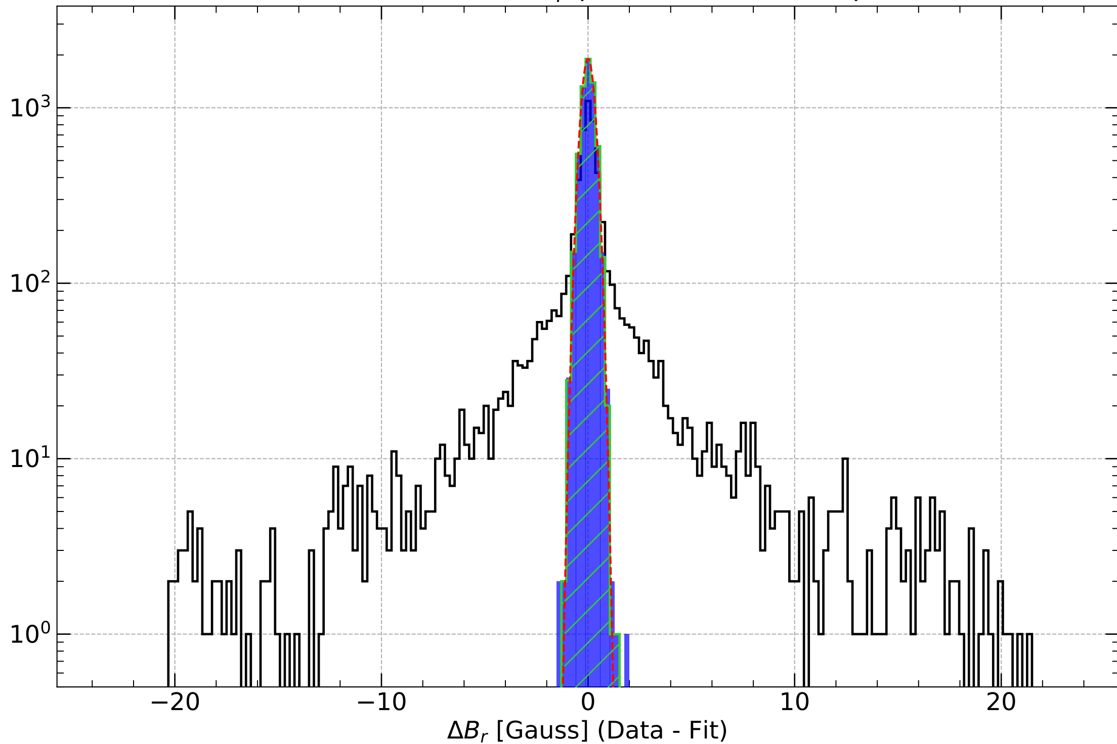
Fit Residuals: \Delta B_r (Measured Dataset)
