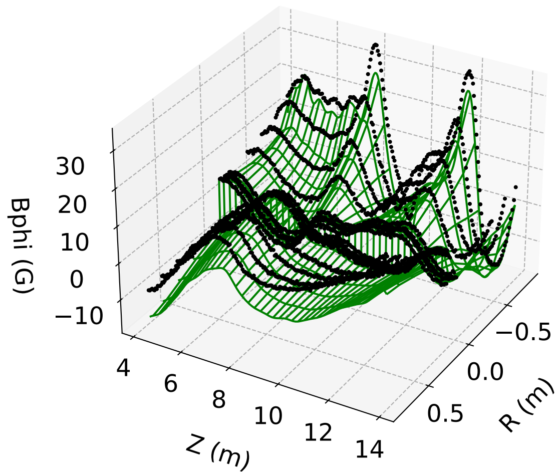
B_\phi vs. r, z ( \phi = 0 ) PINN Model (#4)
