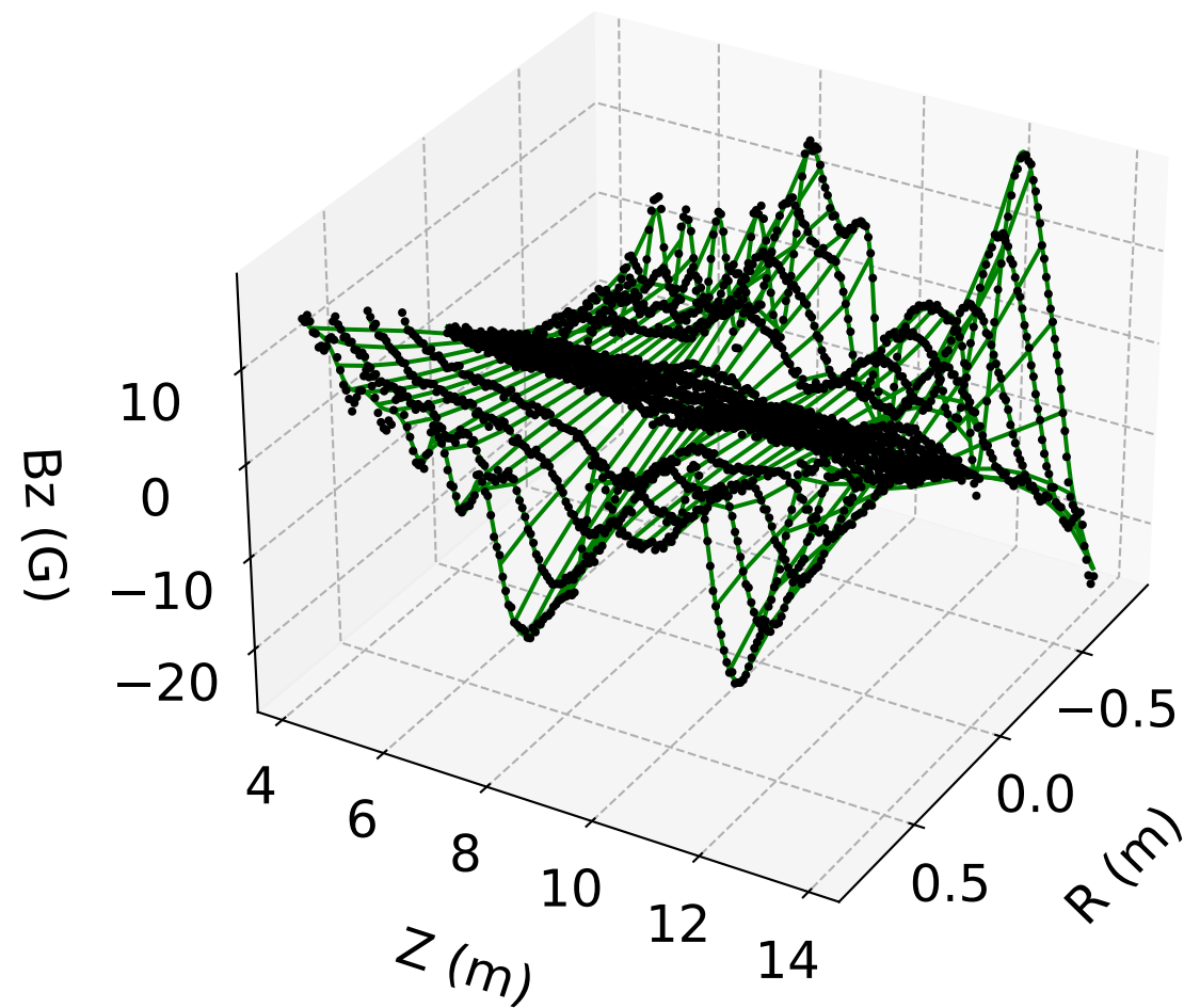
B_z vs. r, z ( \phi = 0 ) PINN Model (#4)
