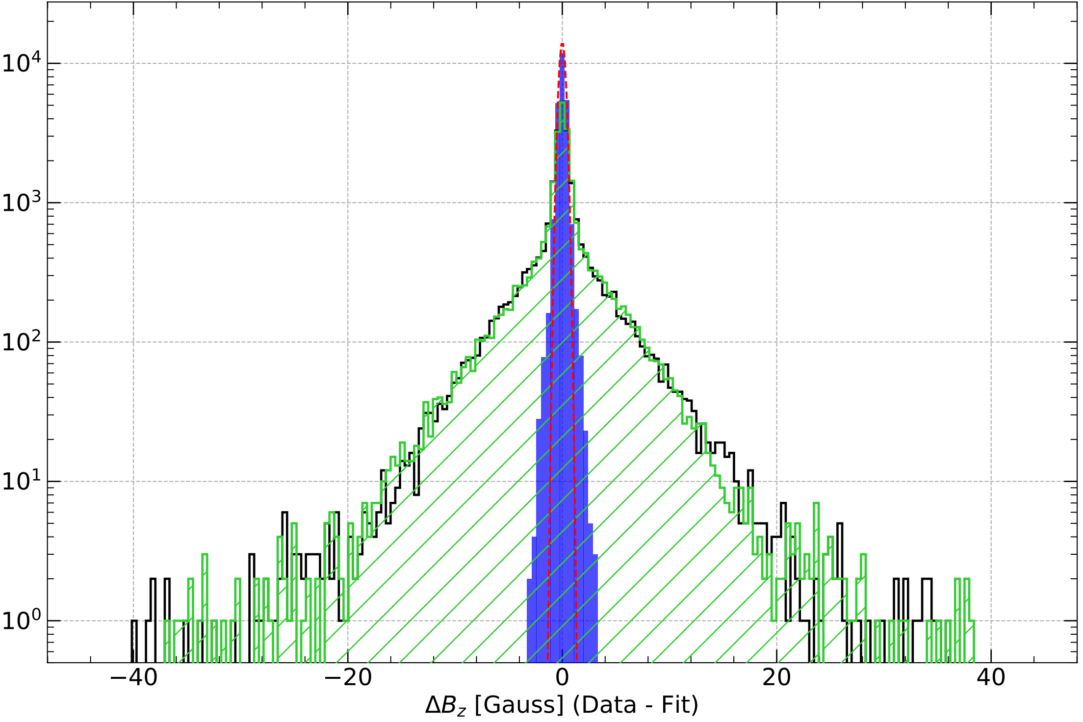
Fit Residuals: \Delta B_z (Measured Dataset)
