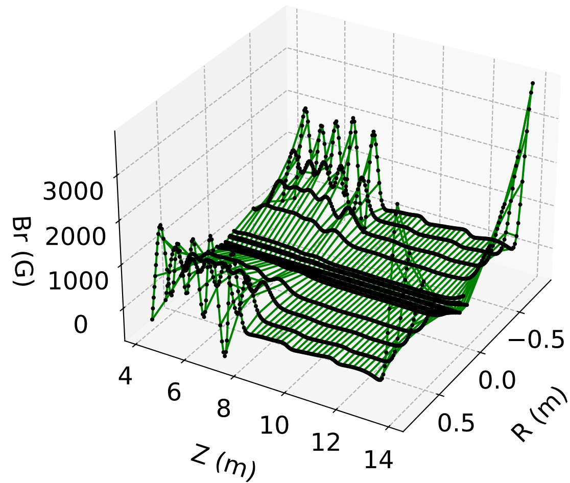
B_r vs. r, z ( \phi = 0 ) Full Model (#5)
