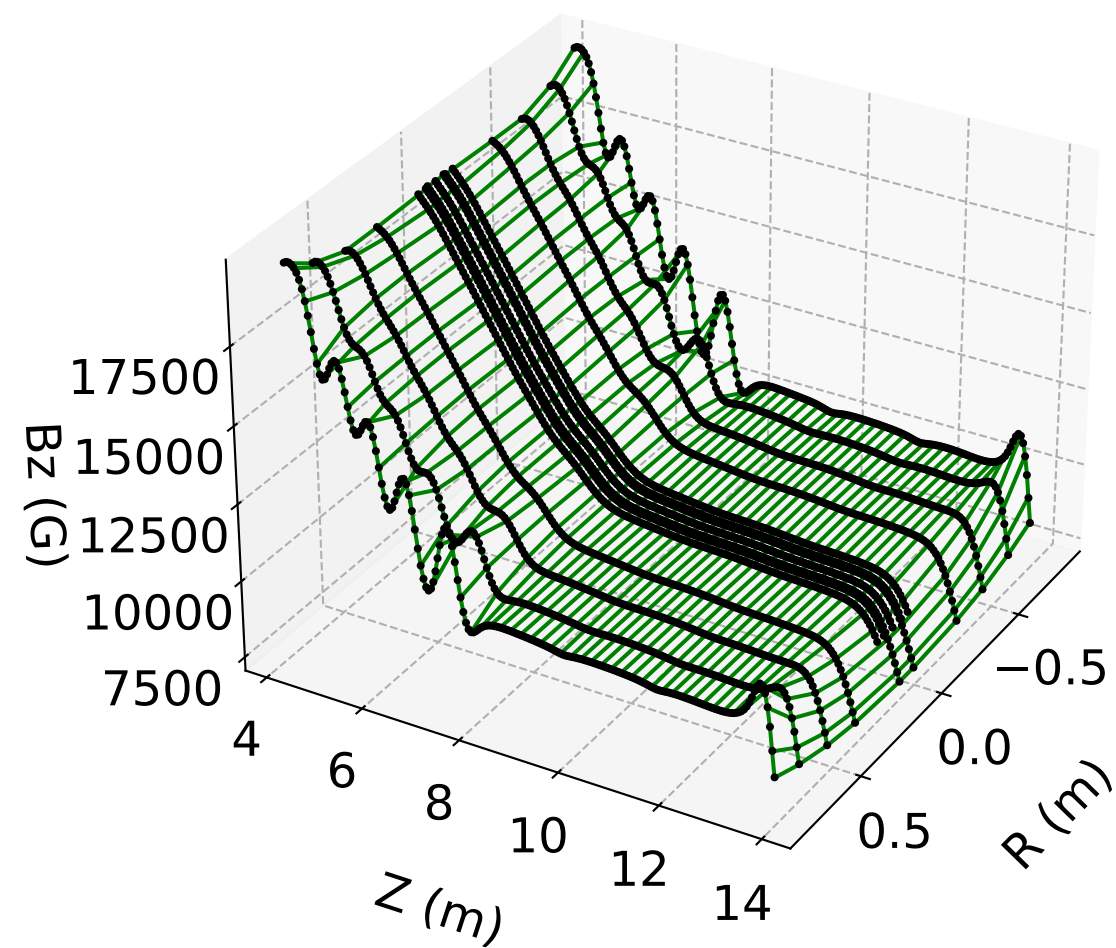
B_z vs. r, z ( \phi = 0 ) LSQ Model (#5)
