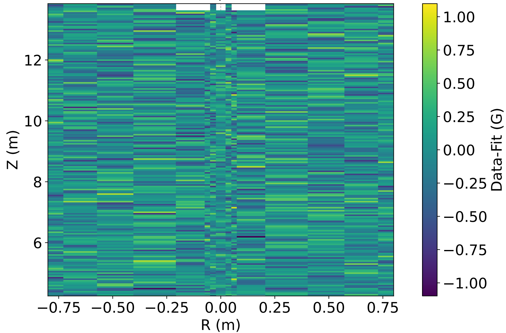
Residual, Data-Fit
