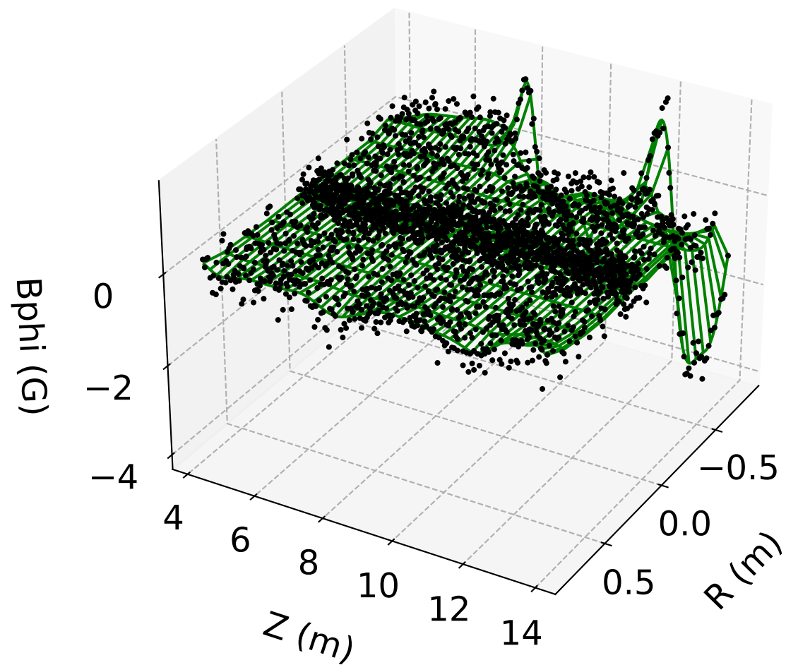
B_\phi vs. r, z ( \phi = 0 ) PINN Model (#8)
