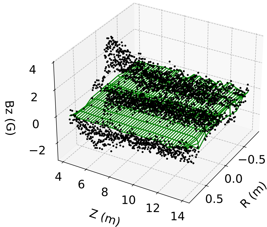
B_z vs. r, z ( \phi = 0 ) PINN Model (#8)
