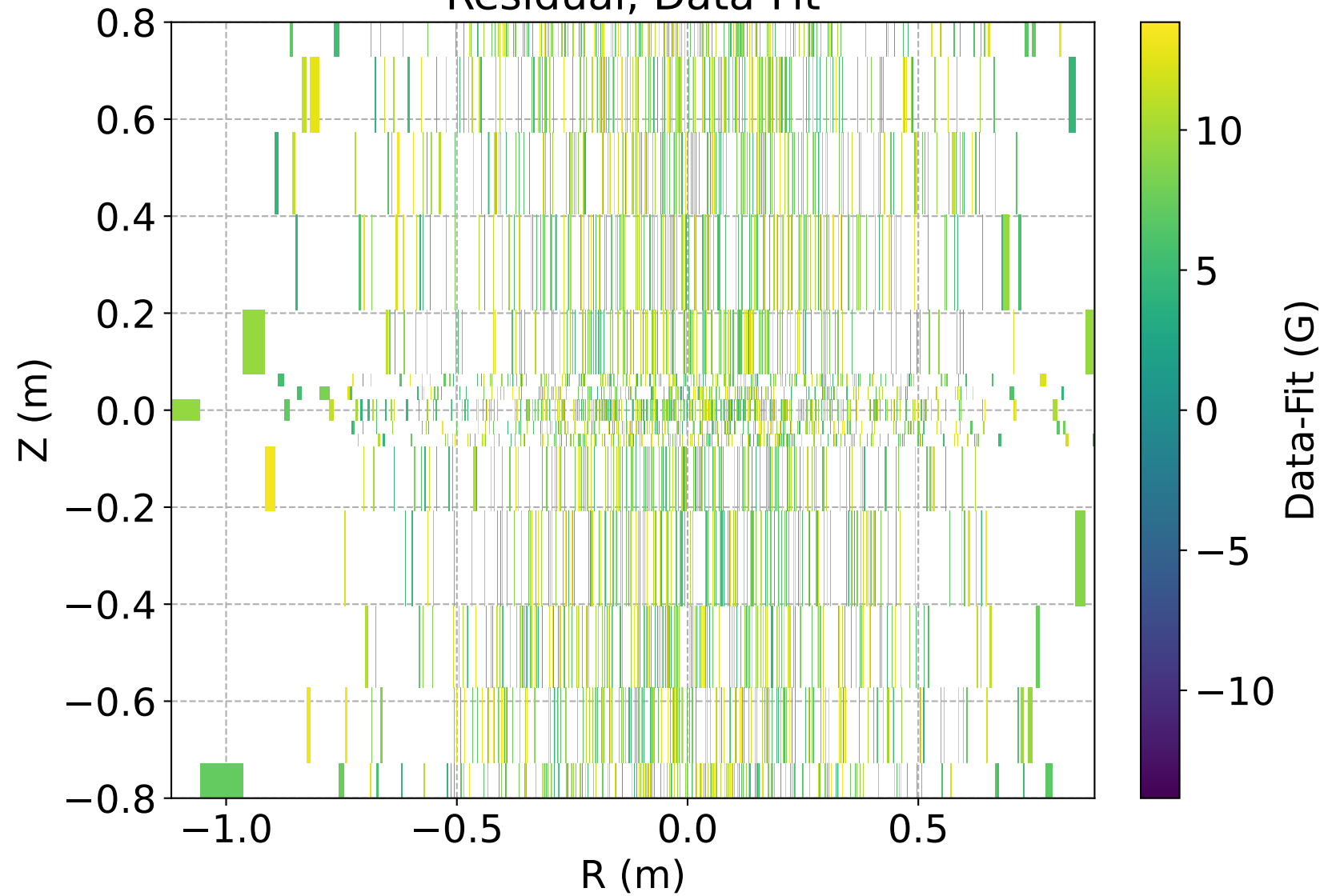
Residual, Data-Fit
