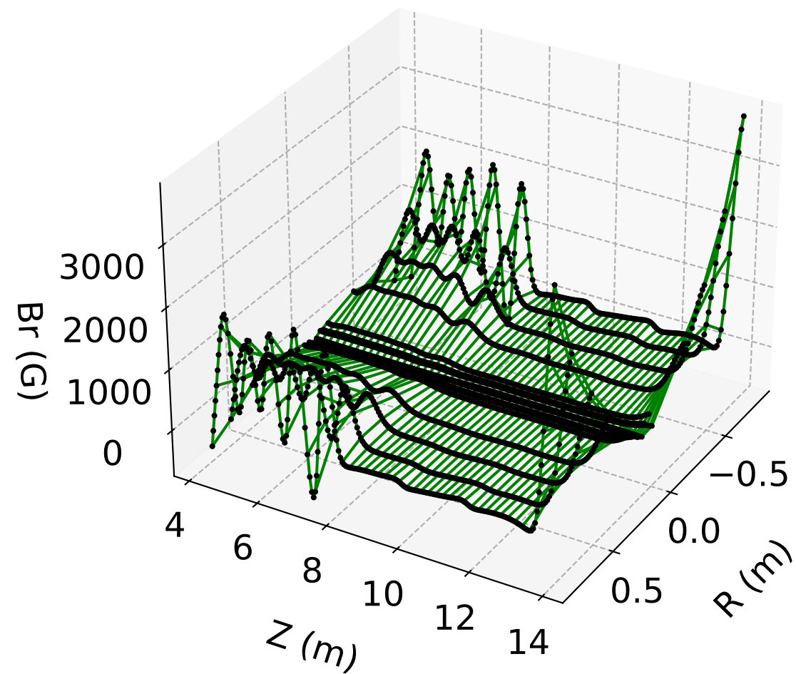
B_r vs. r, z ( \phi = 0 ) LSQ Model (#1)
