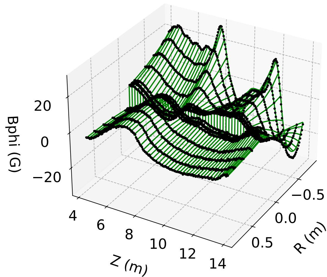
B_\phi vs. r, z ( \phi = 0 ) LSQ Model (#1)
