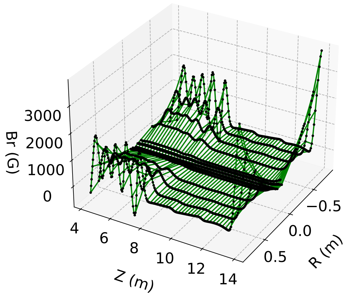
B_r vs. r, z ( \phi = \pi/2 ) Full Model (#1)
